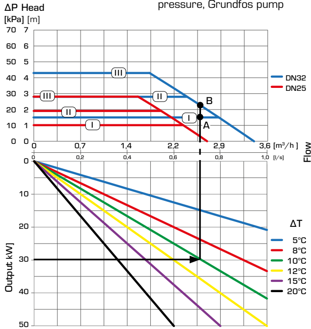
SERIES GRA212, GRA232 – Constant differential pressure, Grundfos pump
