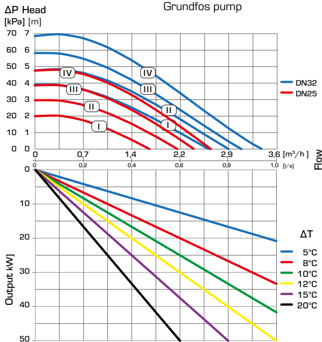
SERIES GRA212, GRA232 – Constant speed, Grundfos pump
