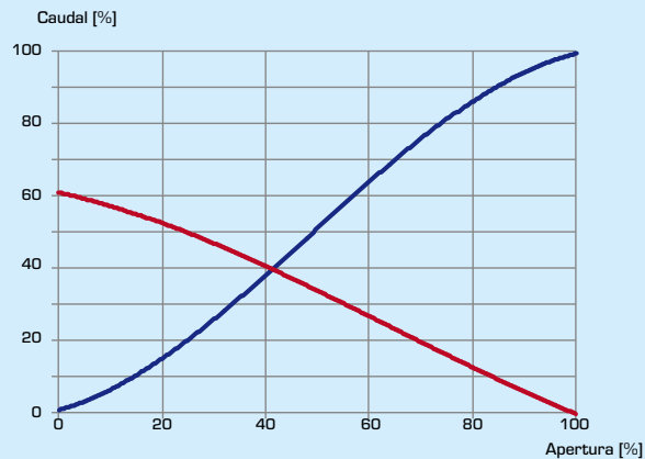
VLG132/VLG142, Kv 2,5, 4
